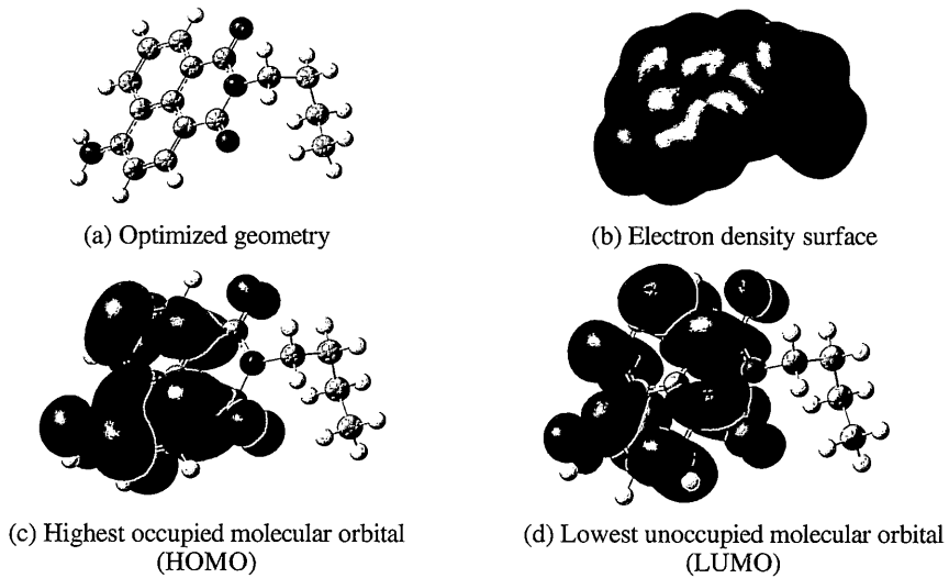
Figure 11. Characteristics of naphthalamide derivative
